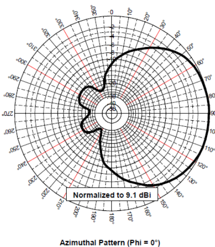
ANTENNA RADIATION PATTERN
