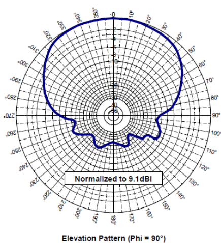
ANTENNA RADIATION PATTERN
